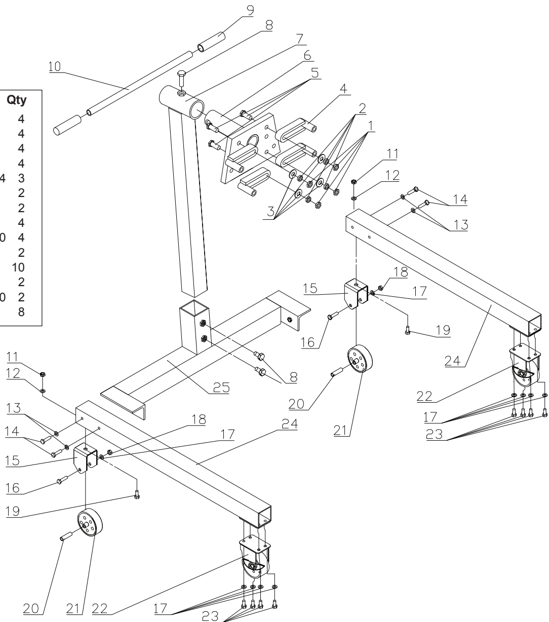
Figure 5 - Assembly Illustration for Model 31250
