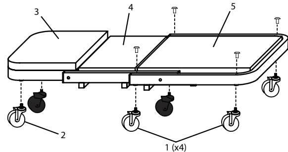
Figure 4 -91000 Parts Breakdown
