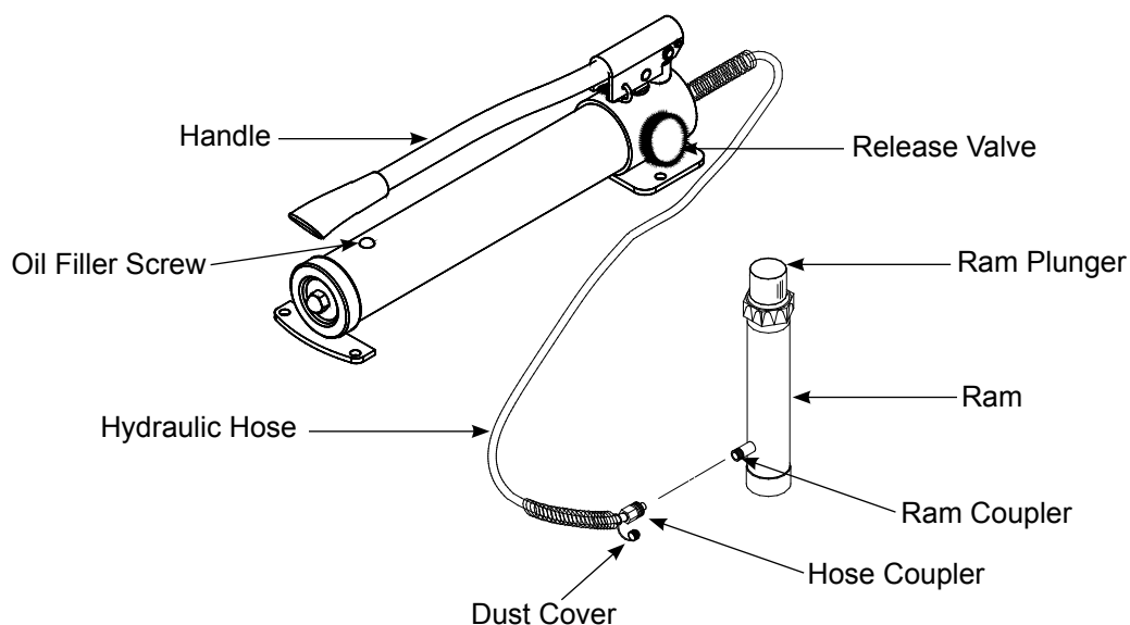
Figure 1 - Pump and Ram Components
