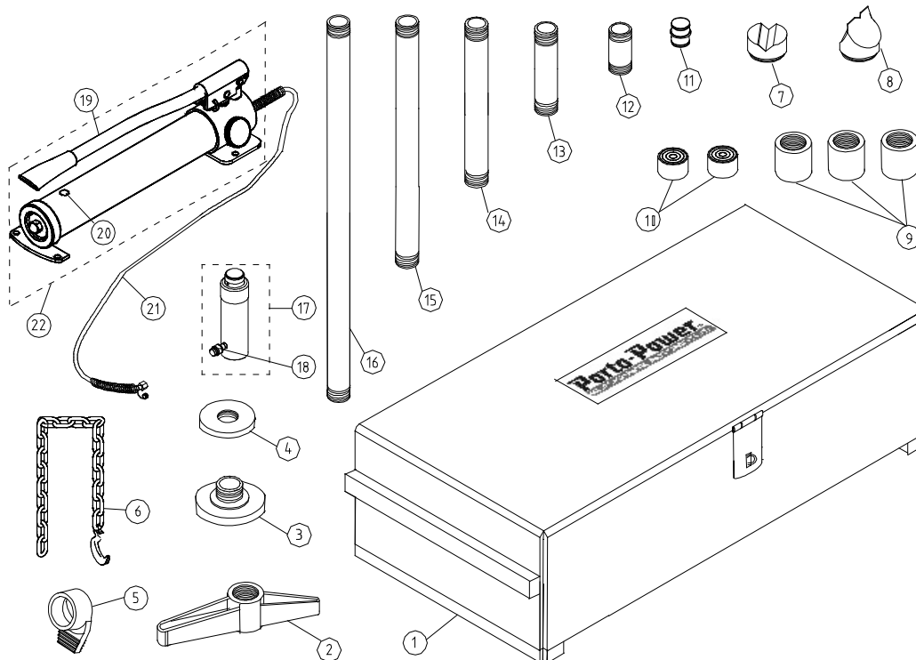
Figure 4 - Replacement Parts Illustration for Model B65041
