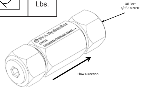
Figure 1: CVC3 Nomenclature
