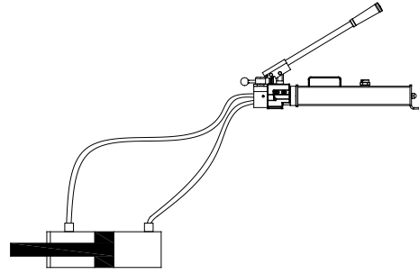
Figure 2 - Illustration to bleed air from system
