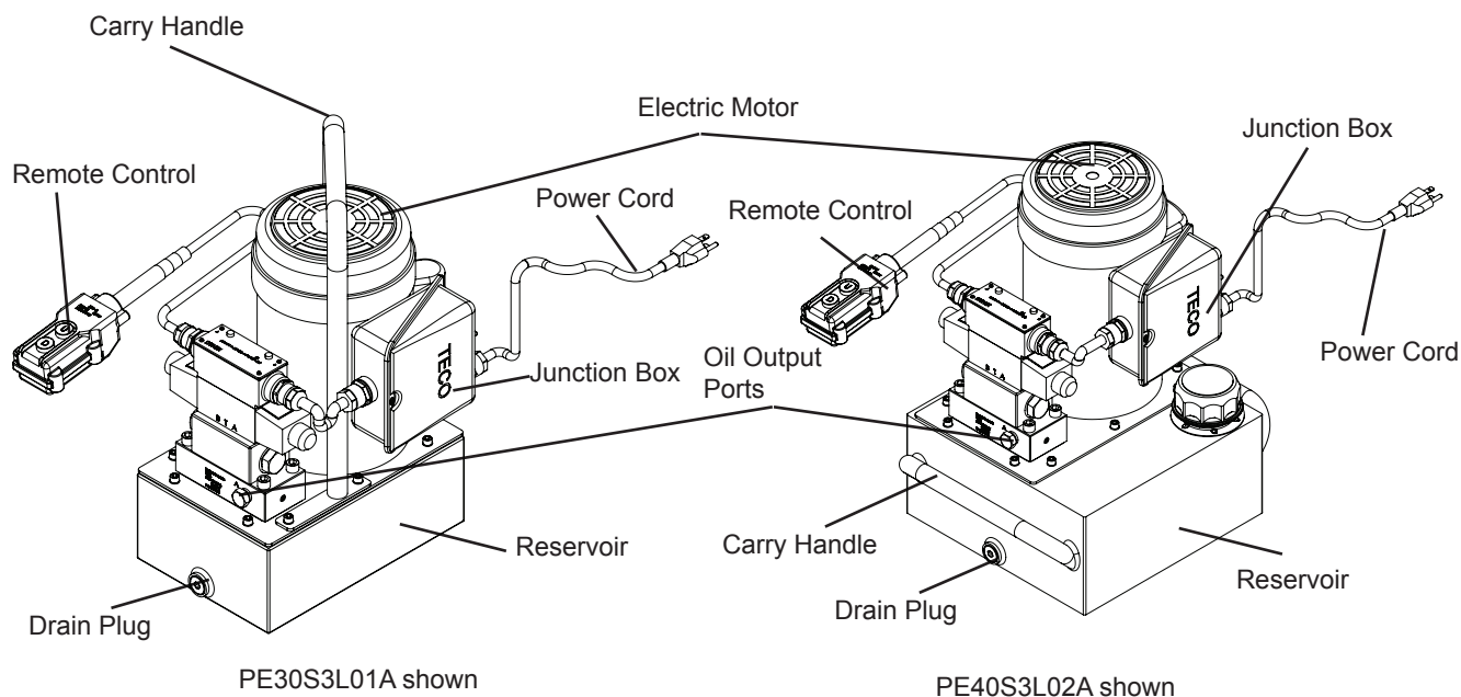
Fig. 1- Electric Pump w/ Solenoid Valve Nomenclature
